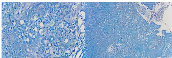
Figure 5. Giemsa Staining
